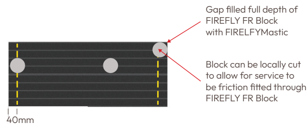
Figure 6 - Penetration allowable zone for SP17 and SP19 in FIREFLY FR Block
