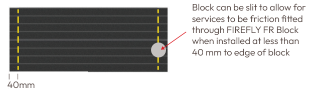
Figure 7 - Penetration allowable zone for services at the edge of FIREFLY FR Block
