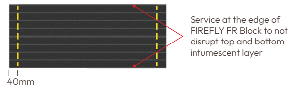
Figure 5 - Penetration allowable zone for FIREFLY FR Block within apertures 500 mm x 200 mm
