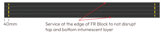
Figure 4 - Penetration allowable zone for FIREFLY FR Block within apertures 1000 mm x 100 mm
