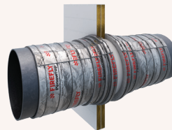
V149 | -/120/120
